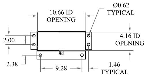
FRONT VIEW SHOWN LESS COVERS
